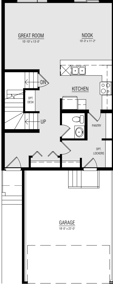
MAIN FLOOR OPTION 726 SQ.FT.
