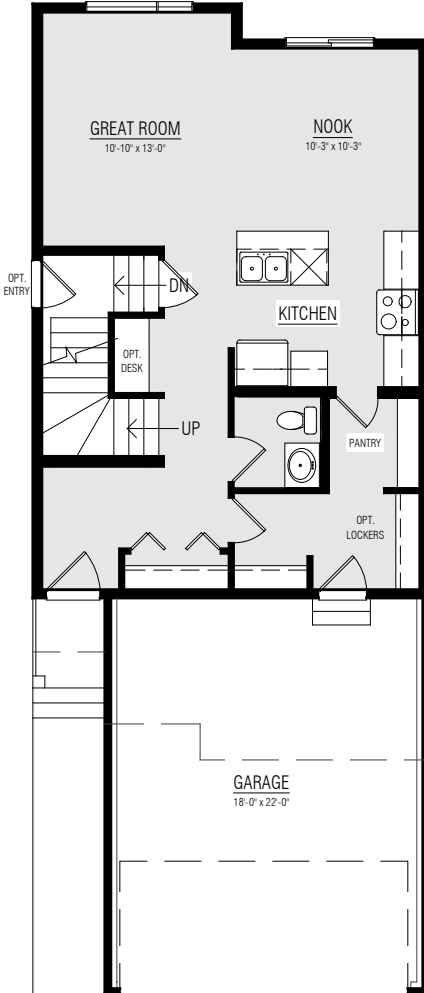
MAIN FLOOR STANDARD 706 SQ.FT.
