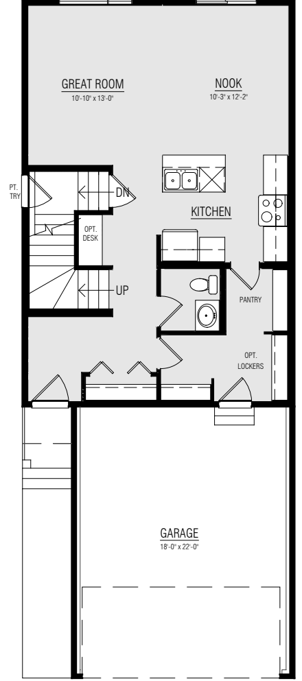
MAIN FLOOR OPTION 726 SQ. FT.
