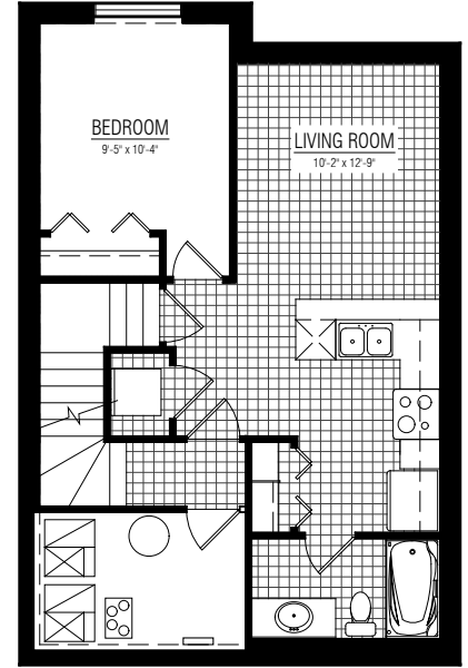
BASEMENT SUITE DEVELOPMENT 560 SQ. FT.
